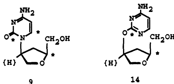
Figure 2. Representative results of 1D J -modulated selective INEPT ^1\text{H} - ^{13}\text{C} NMR correlations (irradiations are depicted as {H} and three bond carbon correlations as *).
