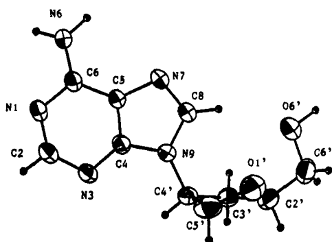
Figure 1. ORTEP plot showing the structure, configuration, and conformation of compound 5.
